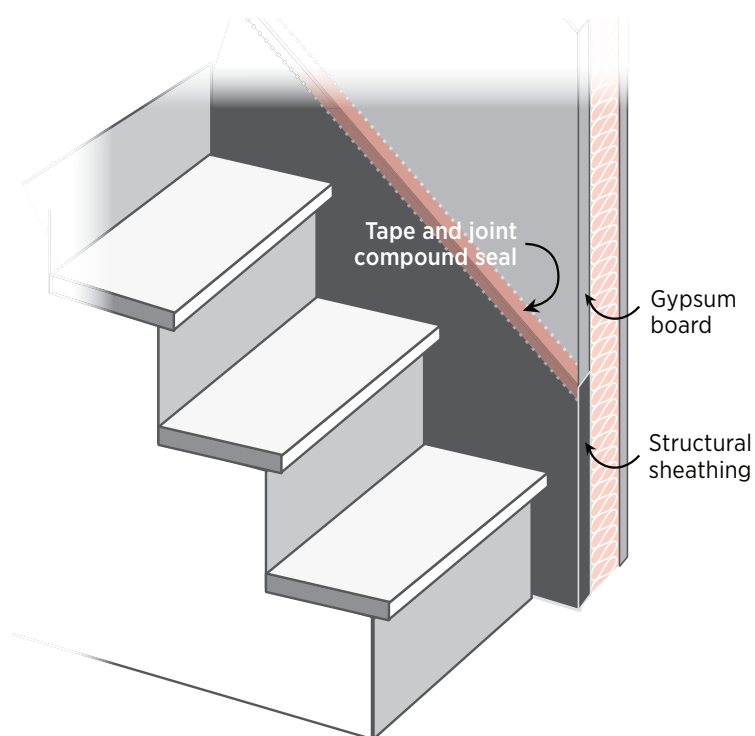
Figure 6.1. Install an air barrier and air sealing on exterior walls behind stairs. If the area behind the stairs is inaccessible, caulk stairs where they meet the wall. Use caulk if the area is already painted; use tape and joint compound if area will be painted.
