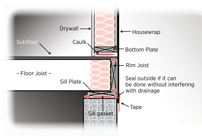
Figure 17.1. Use caulk or spray foam to air seal where the foundation wall meets the sill plate, where the sill plate meets the rim joist, and where the rim joist meets the subfloor.
