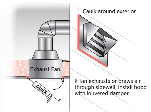
Figure 13.4. Caulk around exhaust fans at the ceiling and exterior wall. Also caulk around exterior outlets and light fixtures.
