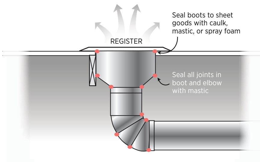
Figure 11.2. Mastic seal all supply and return air ducts.
