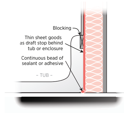
Figure 13.2. If you are remodeling a bathroom make sure you seal and insulate behind the tub or shower, especially if it is on an exterior wall.
