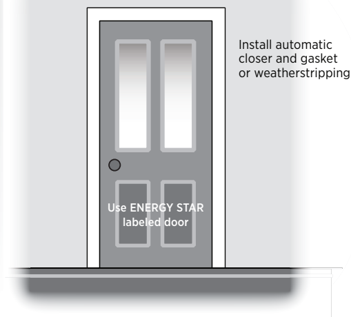
Figure 18.2. Install automatic closer and gasket or weatherstripping around doors. Caulk around trim.
