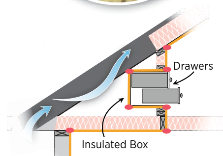
Figure 3.3. Build an airtight, insulated box around any drawers or closets built into attic knee walls that extend into uninsulated attic space. Insulate along air barrier (shown in yellow on drawing) or along roof line with rigid foam (Source: Iowa Energy Center 2008).
