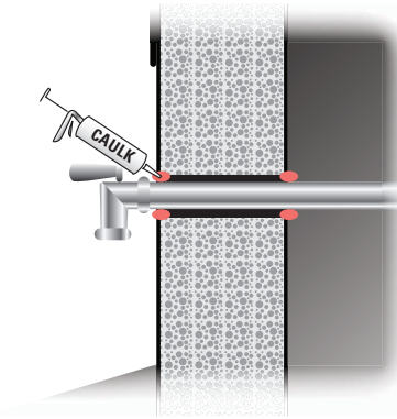
Figure 13.1. Caulk all plumbing penetrations through exterior walls.
