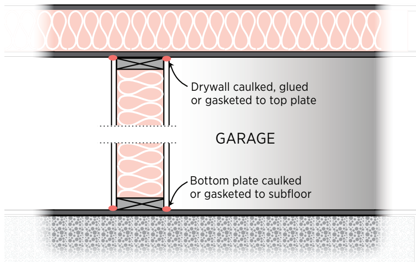
Figure 15.1. Finish the walls that separate the garage from the rest of the home with drywall that is sealed to the top and bottom plate with a bead of caulk.
