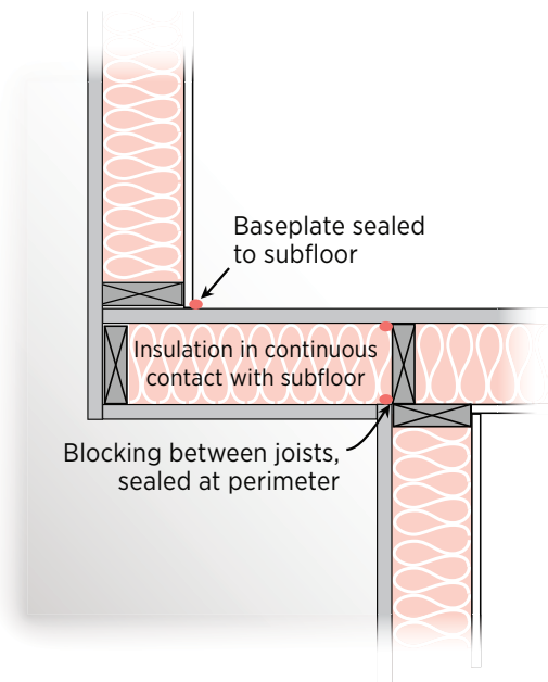
Figure 16.1. Block and air seal both the floor-to-upper wall junction and the floor-to-lower wall junction.
