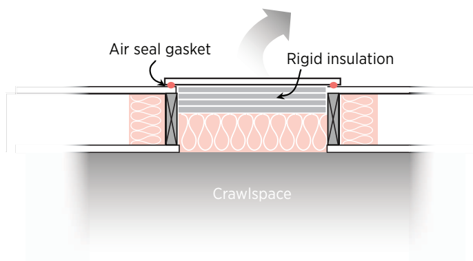
Figure 17.3. Air seal the crawlspace access hatch by installing a gasket or weather stripping around the hatch edges.
